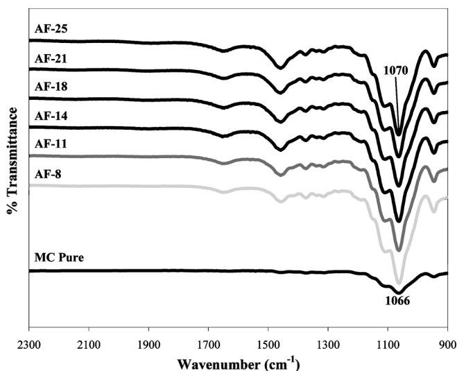
Figure 2. FT-IR spectrum of the sample in the region between 900 and 2300 \text{cm}^{-1} .
